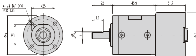
GEARHEAD LENGTH
